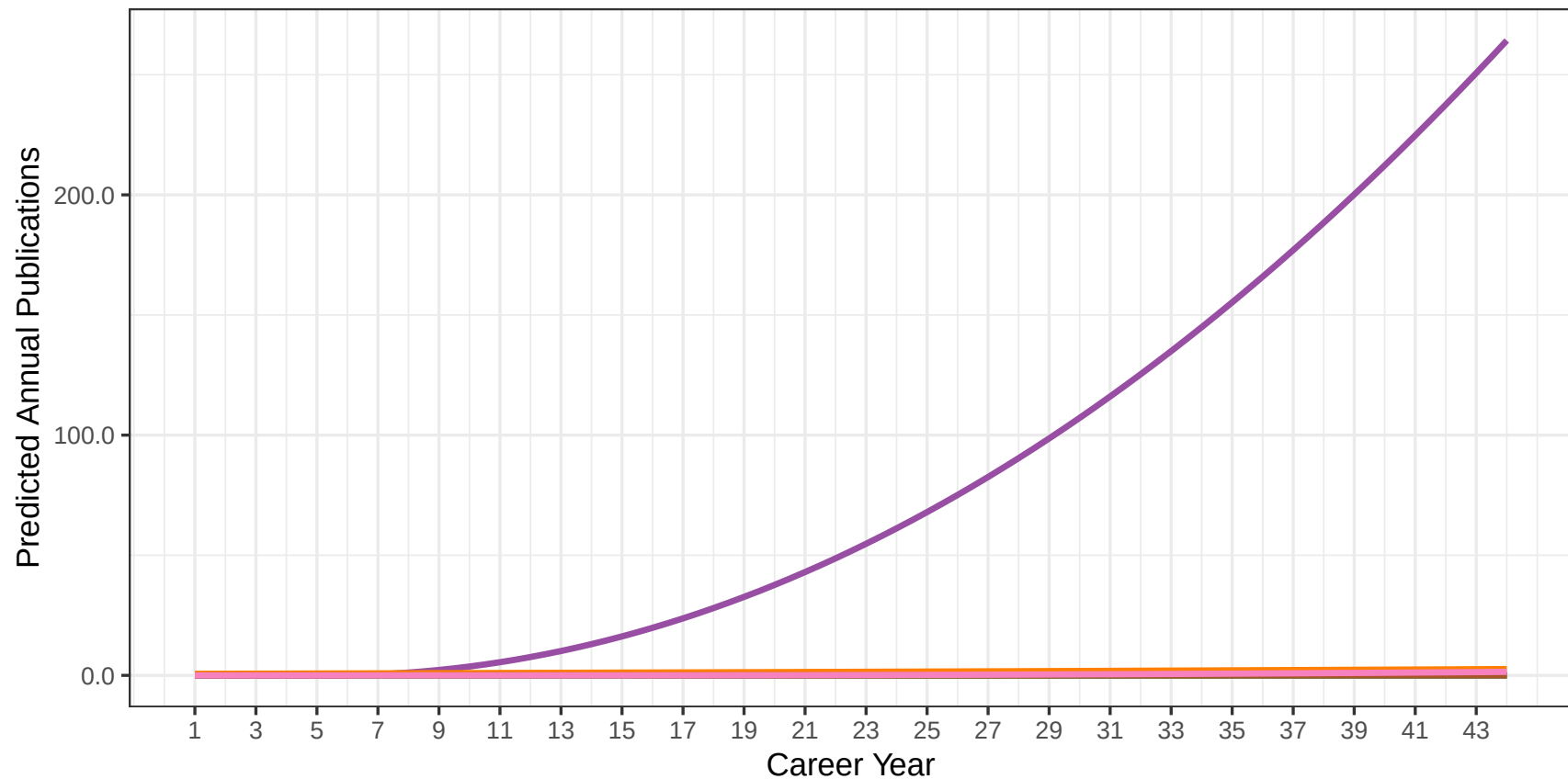
LCGA Publication Trajectories (10 Classes, linear growth)
