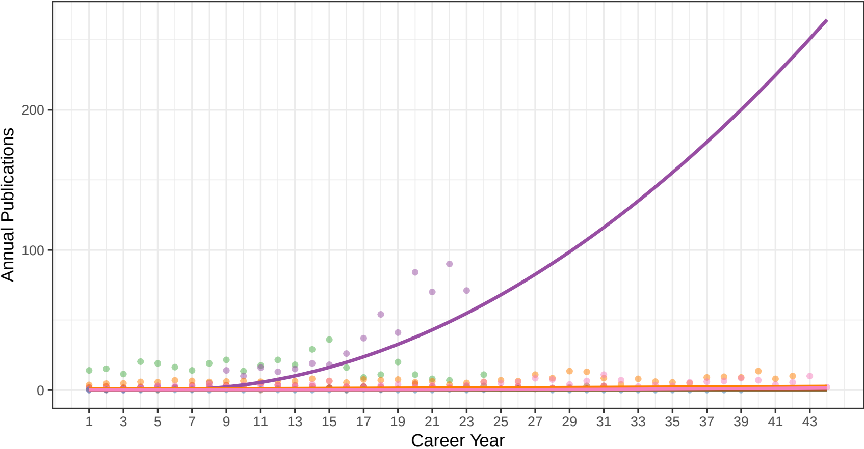
Observed Means (points) vs. LCGA Predicted Trajectories (lines)
